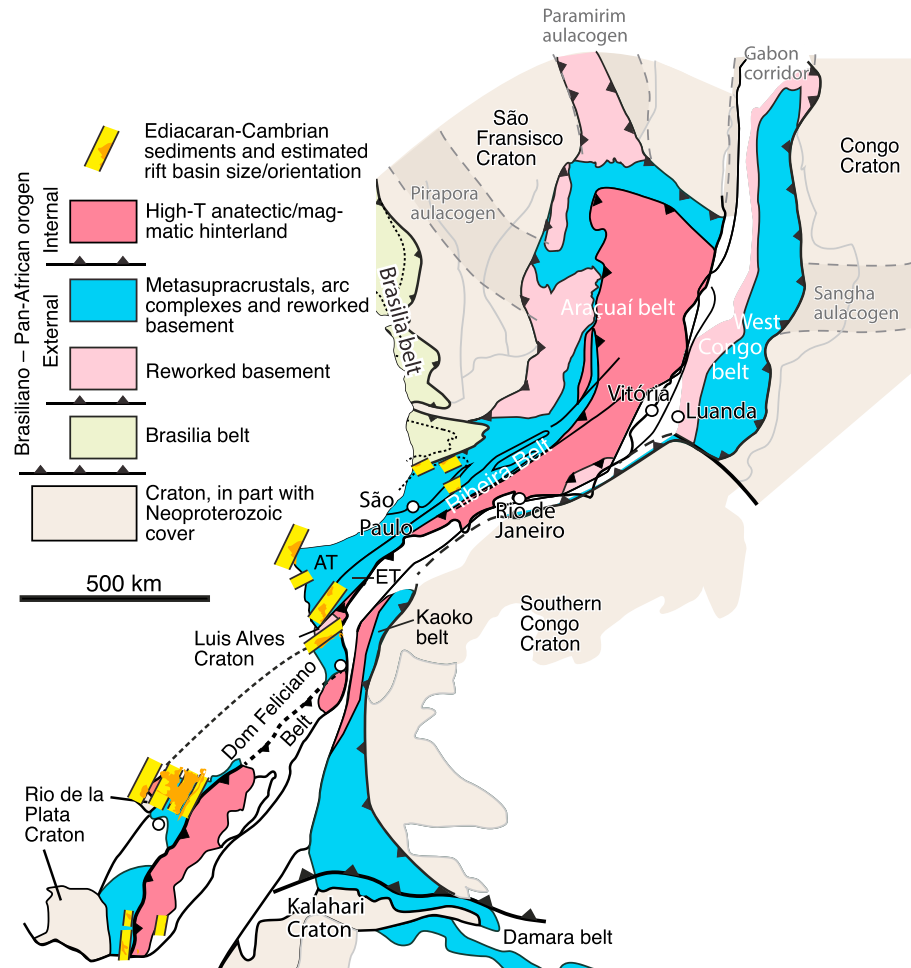
Figure 4. Tectonic map of the Mantiqueira (Araçuaí-Ribeira-Dom Feliciano) orogenic system. Based mainly on Heilbronn et al. (2008), Tack et al. (2001), Pedrosa-Soares et al. (2008), and Almeida et al. (2012). AT = Andrelândia terrane; ET = Embu Terrane.
